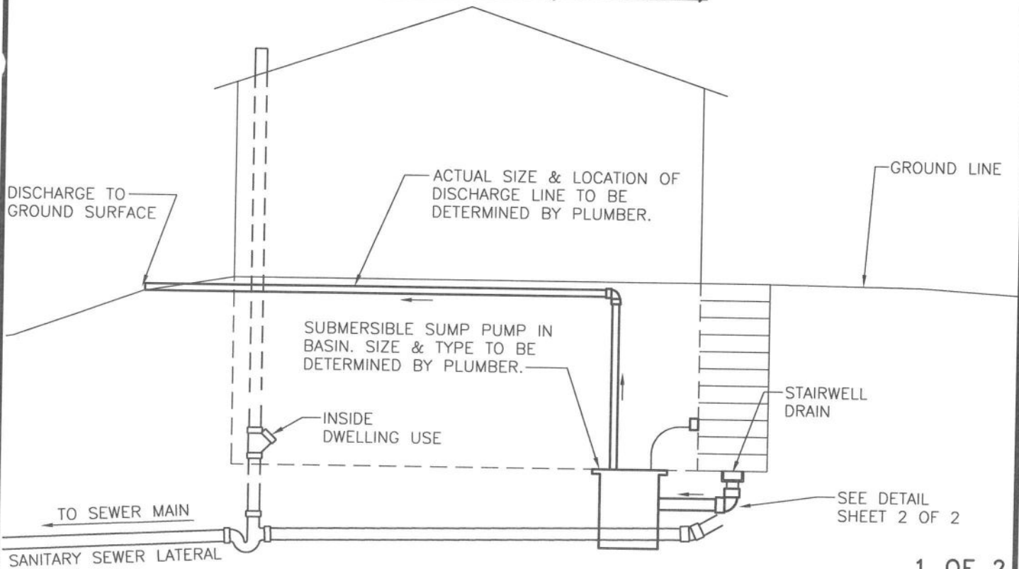
TYPICAL STAIRWELL DRAIN DISCONNECTION WITH SUMP PUMP INSTALLATION
