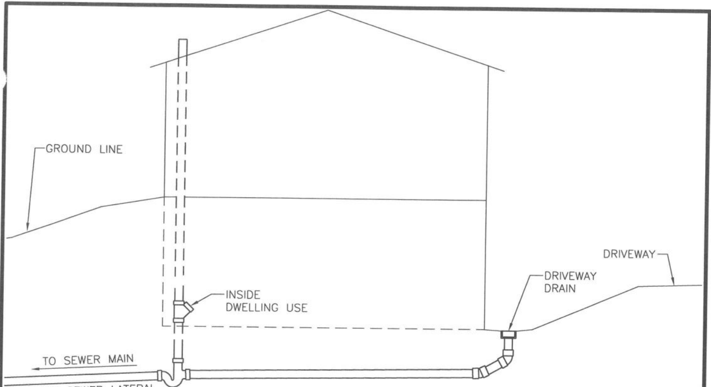
TYPICAL DRIVEWAY DRAIN CONNECTION TO SANITARY SEWER (PROHIBITED)
