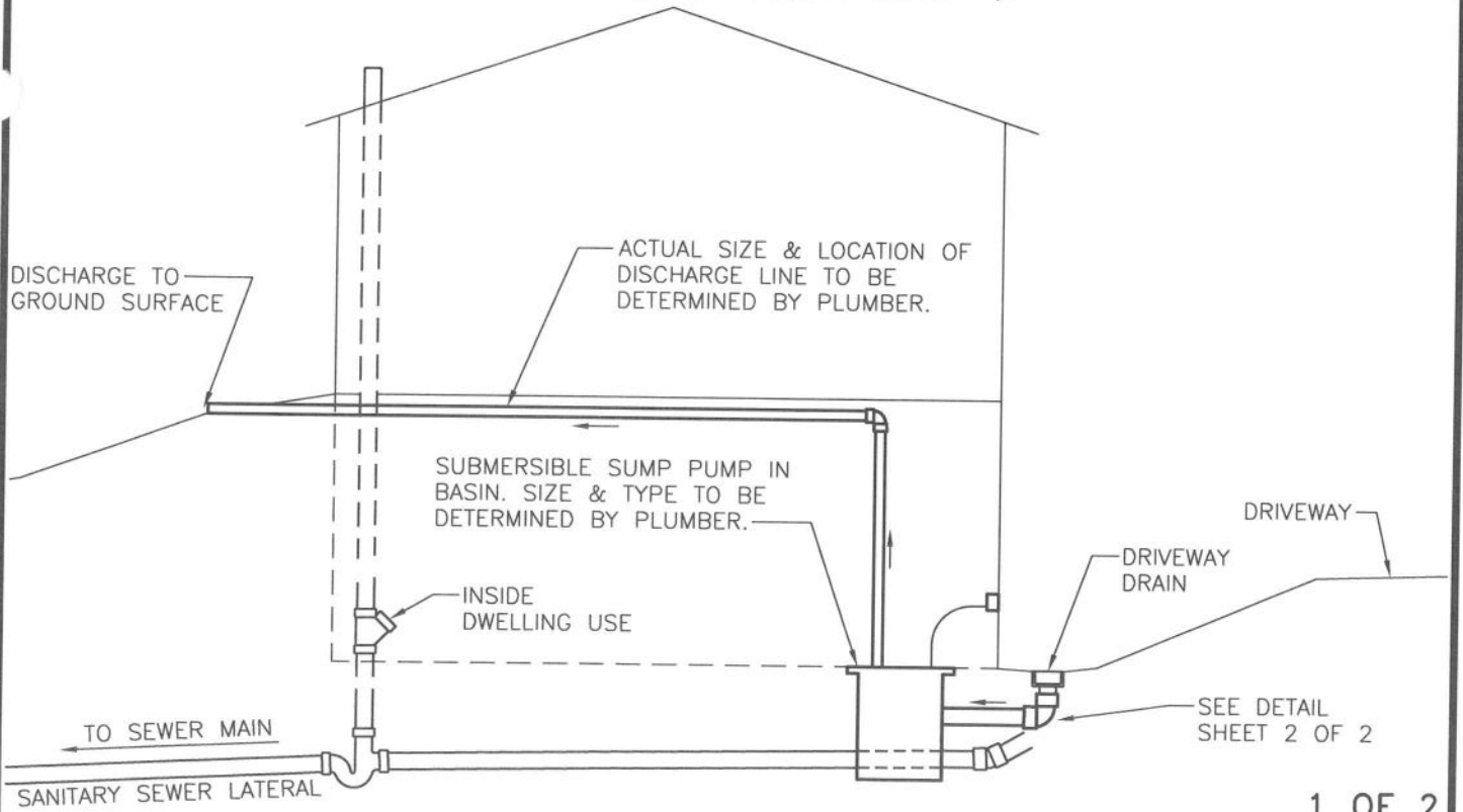
TYPICAL DRIVEWAY DRAIN DISCONNECTION WITH SUMP PUMP INSTALLATION
