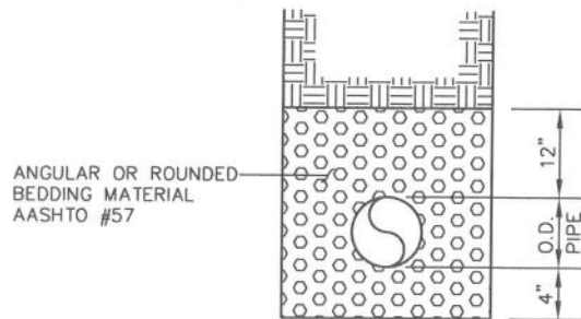
TRENCH SECTION
