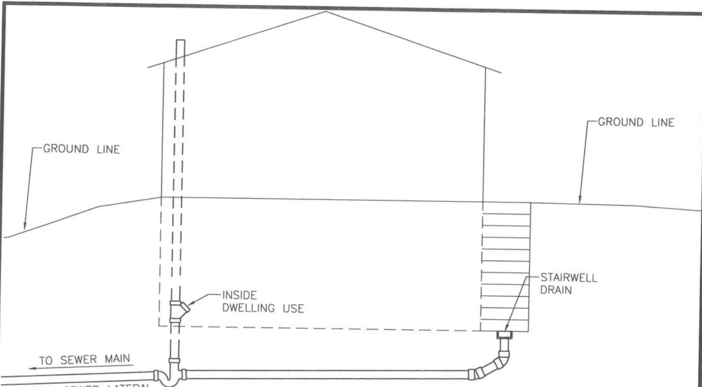
TYPICAL STAIRWELL DRAIN CONNECTION TO SANITARY SEWER (PROHIBITED)
